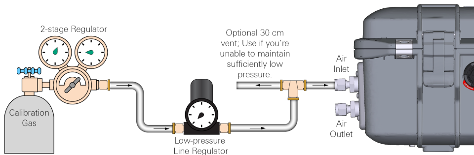
Figure 6-1. Plumbing configuration for calibration gases. Use a low pressure regulator to reduce pressure and a 30 cm vent to are recommended avoid pressurizing the inlet.
