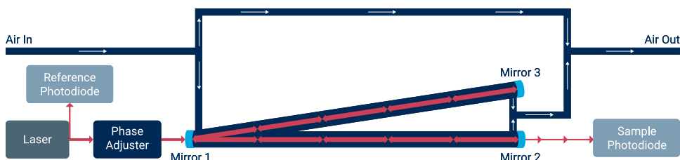
Figure A-1. Simplified schematic of the LI-7815 flow path through the optical bench. The phase adjuster is a volume in the path between the laser and optical bench that is tied to a pressure control mechanism. Changing the pressure of that volume alters the refractive index which subsequently modifies the phase of the laser.
